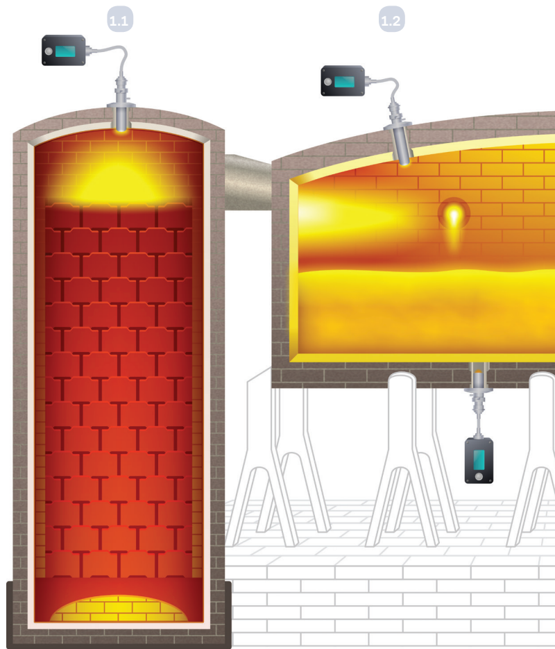
Regenerator
