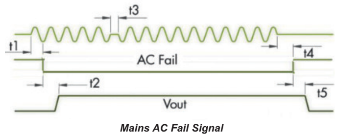
Mains AC Fail Signal
