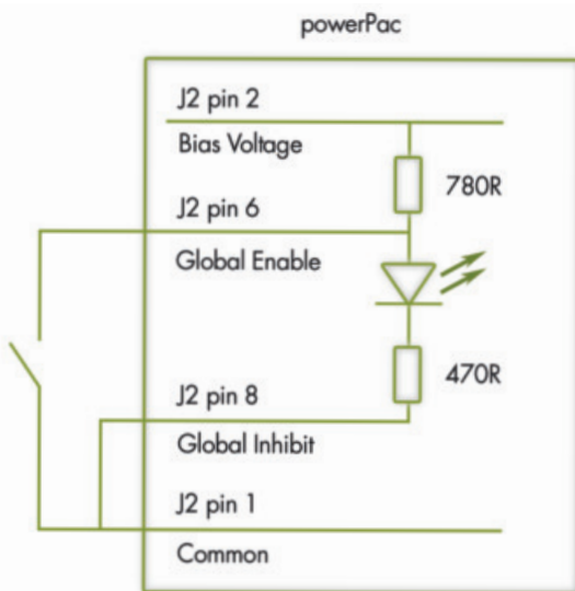
Global Enable Using Bias Supply Voltage
