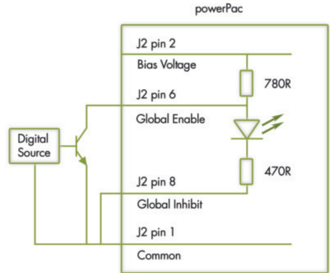
Global Enable Using an External Signal
