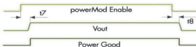
Output powerMod Signals
