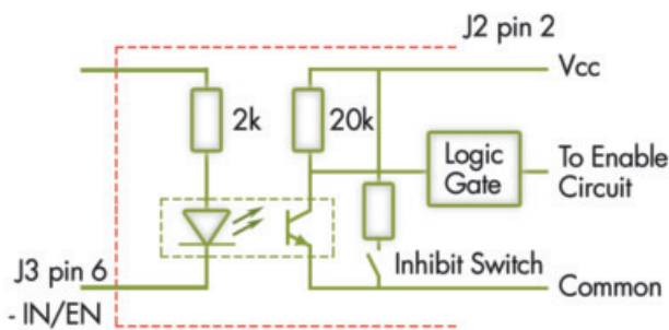
Remote Inhibit/Enable of Output
