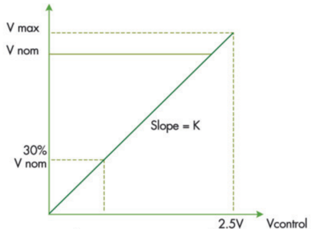
Remote Output Voltage Adjustment of powerMods
