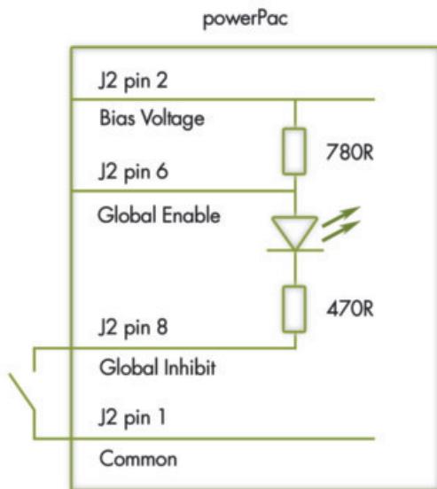
Global Inhibit Using Bias Supply Voltage
