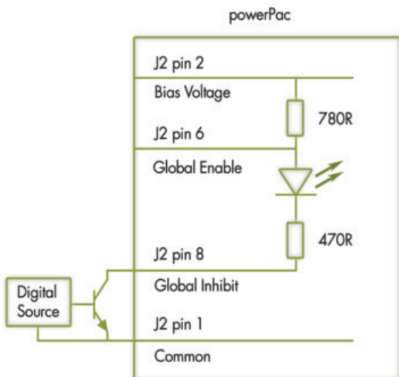
Global Inhibit Using an External Signal
