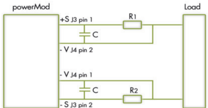
Remote Sense of Output Voltage
